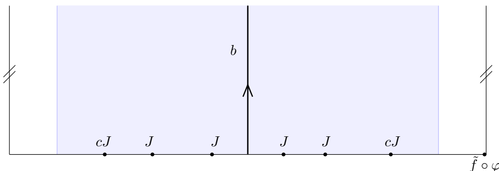
Figure 3: The geometric definition of the states |\theta_n\rangle . The distance between the J 's is integrated from 0 to 1. For convenience, we have also used the fact that B^2 = 0 to reduce the number of b contours to just one, while removing all but two of the c 's.
